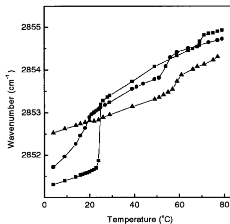
FIGURE 1 Variations of the symmetric \nu_{\text{C-H}} band position as a function of temperature for pure POPE (■), POPE/20 mol % chol (●), and POPE/45 mol % chol (▲).
