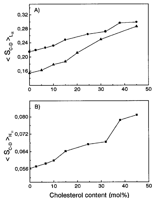
FIGURE 7 Variation of \langle S_{\text{CD}} \rangle as a function of cholesterol content in the lamellar phase (A) for POPE- \text{d}_{31} ( 32^\circ\text{C} ; ●) and POPC- \text{d}_{31} (▲) (from Lafleur et al., 1990a, at 30^\circ\text{C} ) and in the \text{H}_{\text{II}} phase (B) for POPE- \text{d}_{31} ( 70^\circ\text{C} ; ■).
